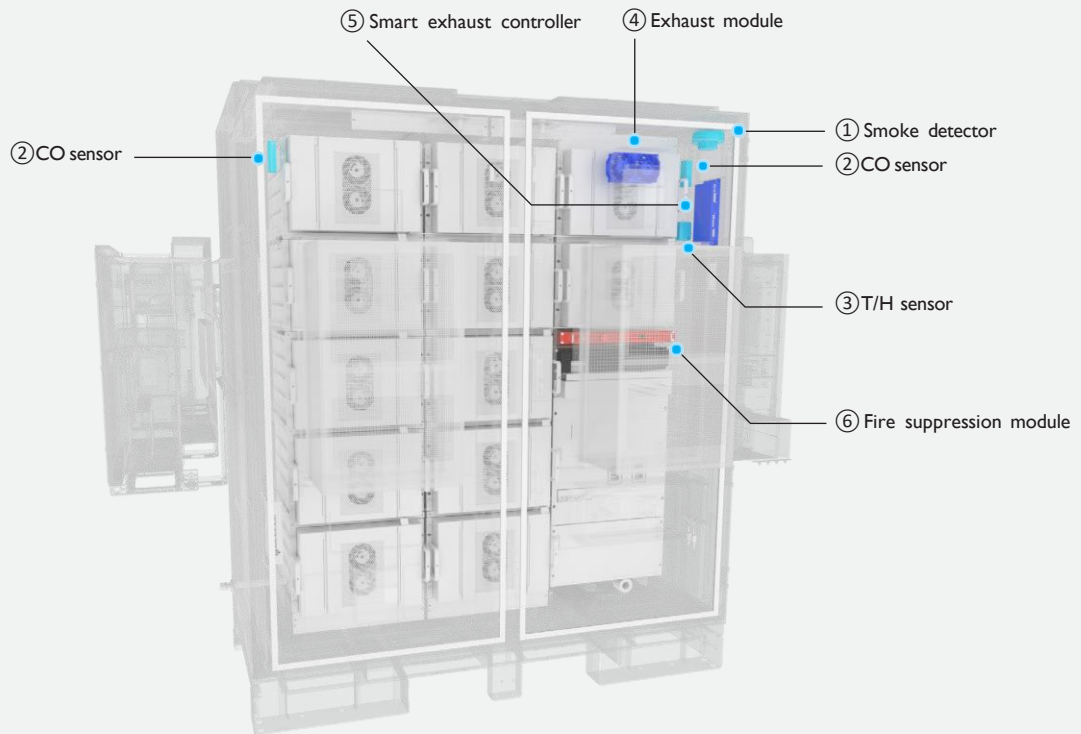
Figure 15. Active fire suppression system
